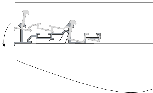
Rail/Riel RM-411
