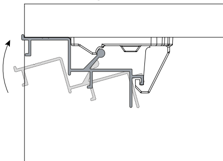
Rail/Riel RM-412
